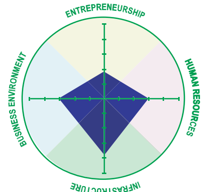
Hussar, Average Score by Variable
